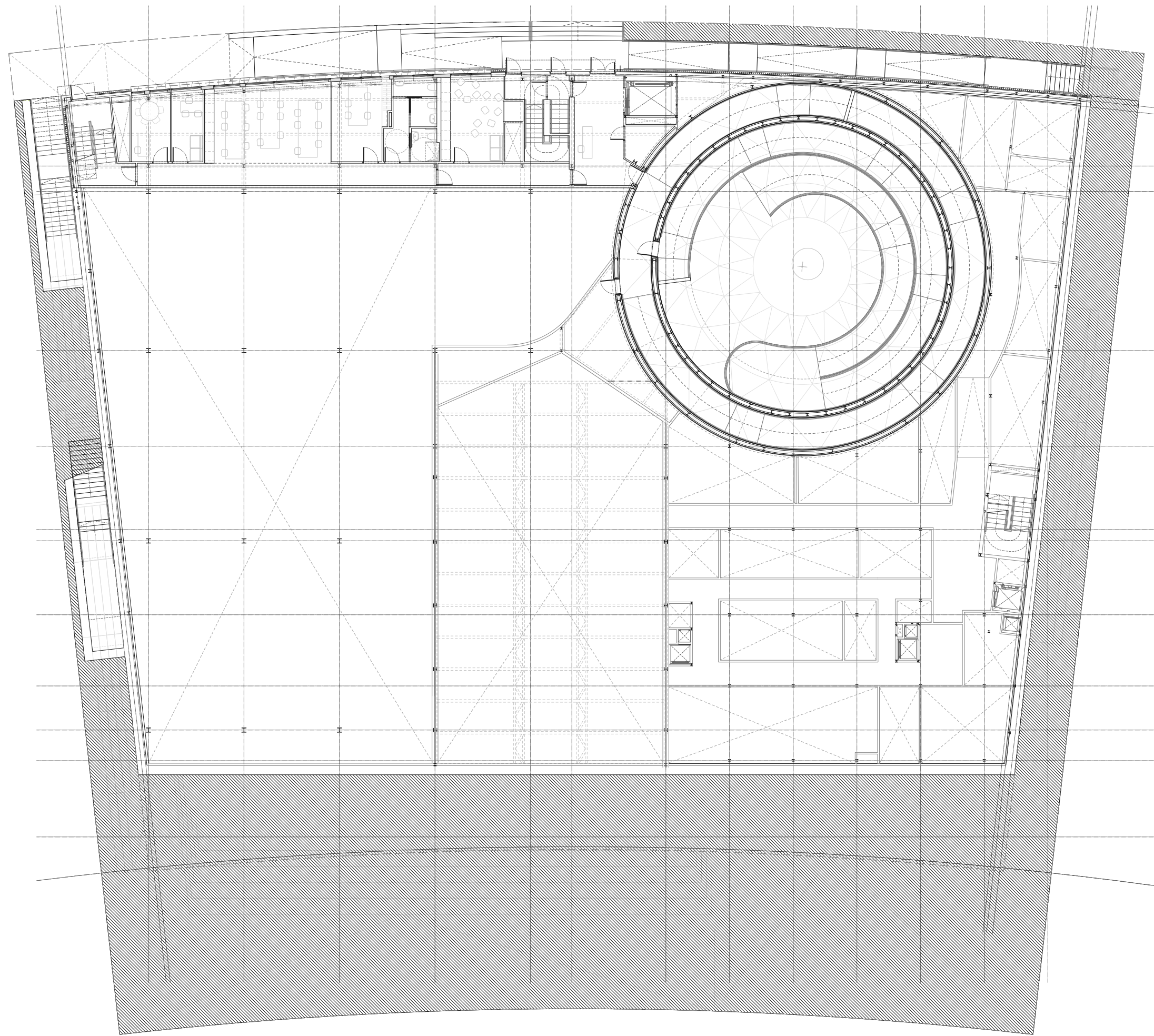
PLANTA MEZZANINE
