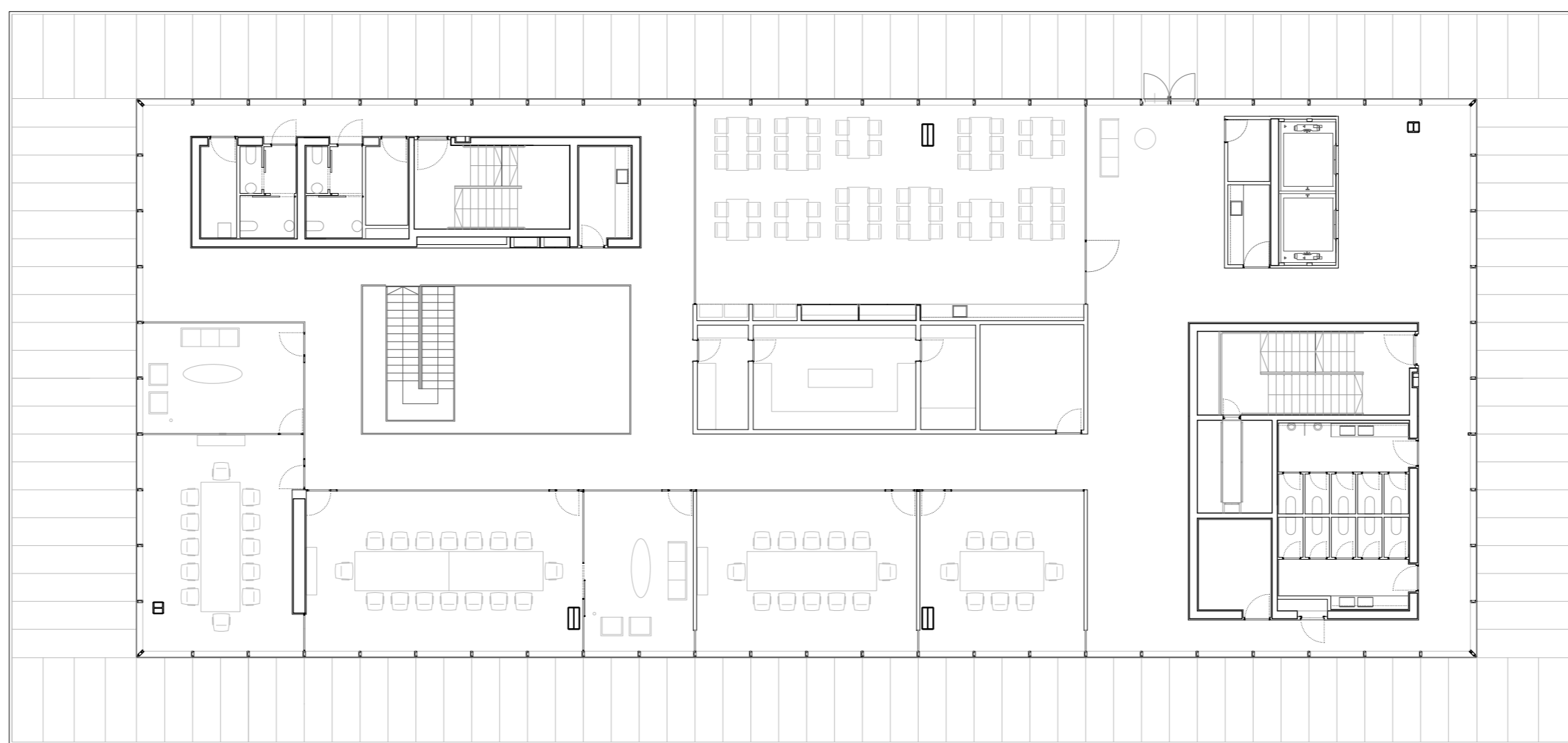
FIRST FLOOR (+4.50m) 0 1 2 5 10
