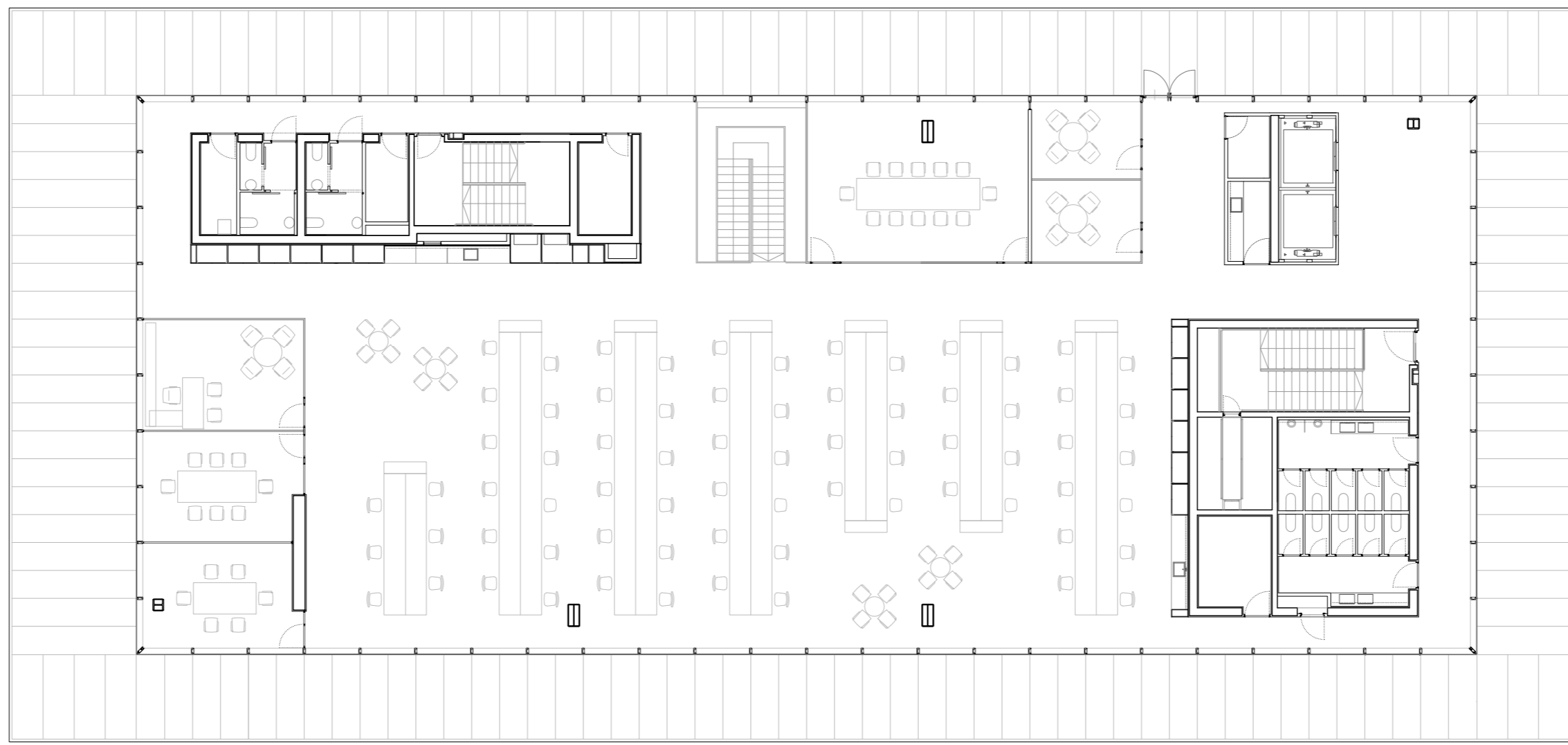
THIRD FLOOR (+13.50m) 0 1 2 5 10
