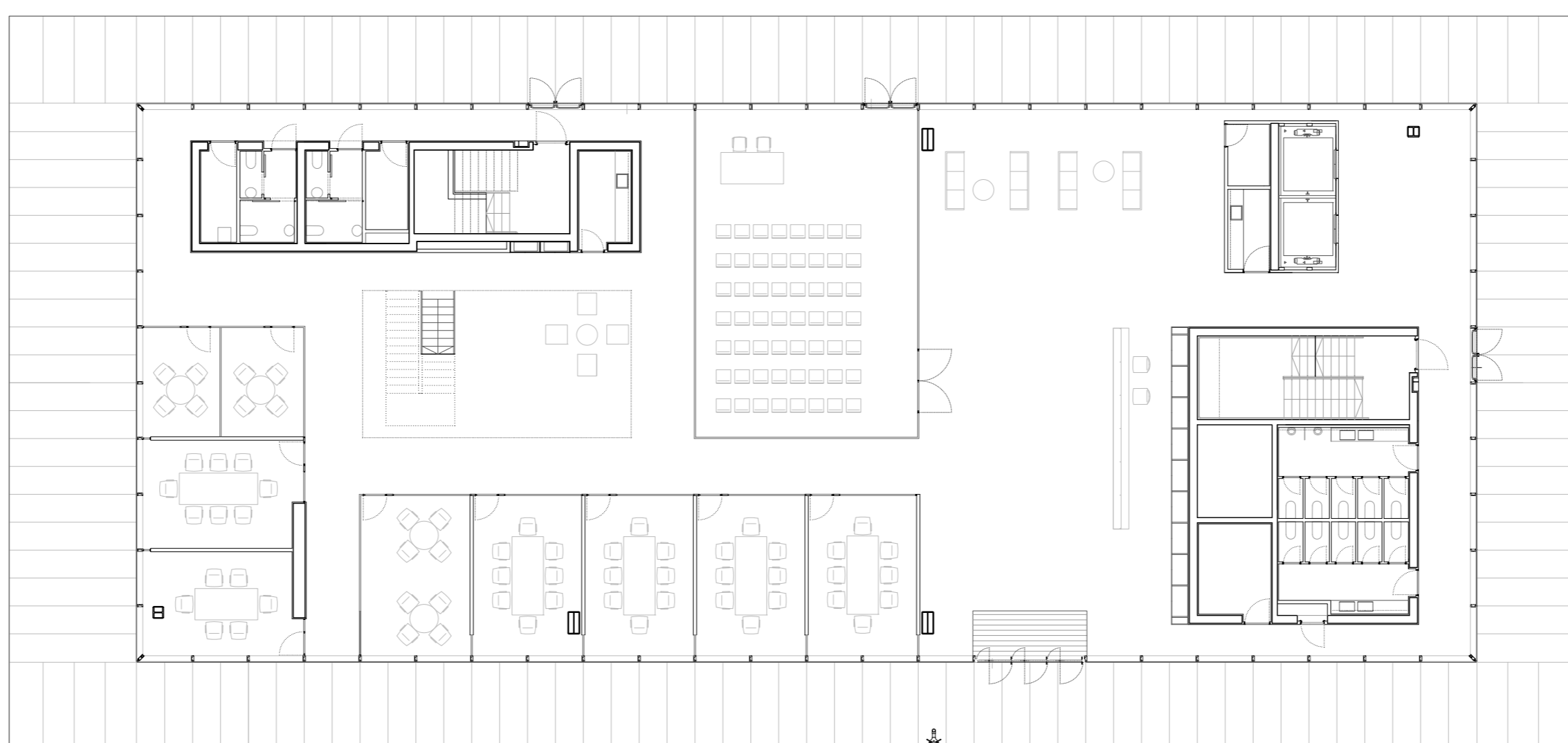
GROUND FLOOR (+0.00m) 0 1 2 5 10
