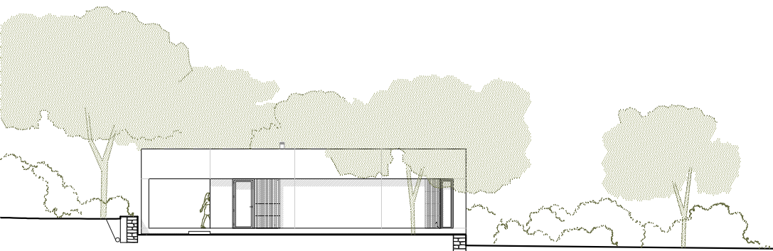
North-West elevation (main building)
