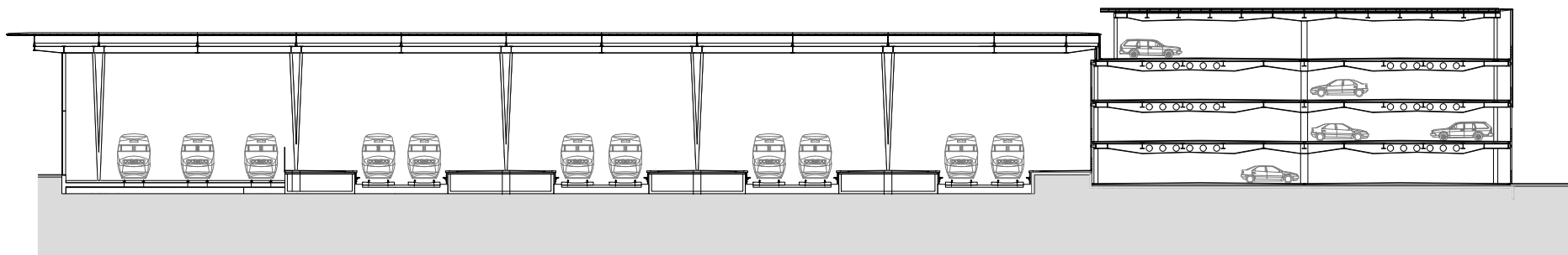
DFA | DIETMAR FEICHTINGER ARCHITECTES - OSTENDE TRAIN STATION - SECTION - ROOF PARKING
