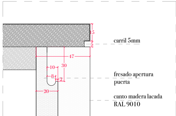
d1.detalle carril de 5mm
