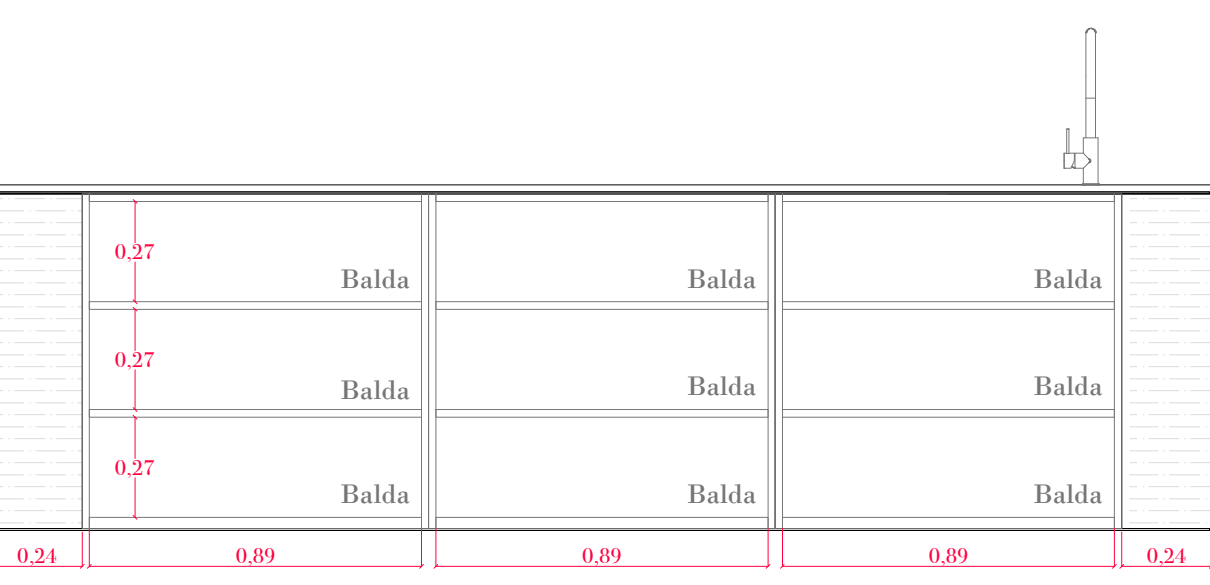
Alzado exterior 2-2´
