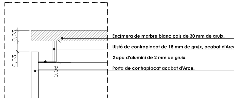
DETALL 1 E:1/5
