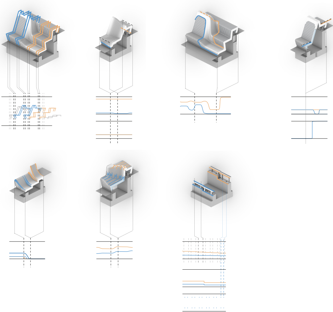
All control curves defining the design, including cross sections, bottom edge, glass/composite overlap, pullback of lamellas, fillets, division of lamellas, structure, concrete foundation and position of fitting bolts (top), with seven selected examples of their effect (bottom). Example of fillet transformation (right page).
