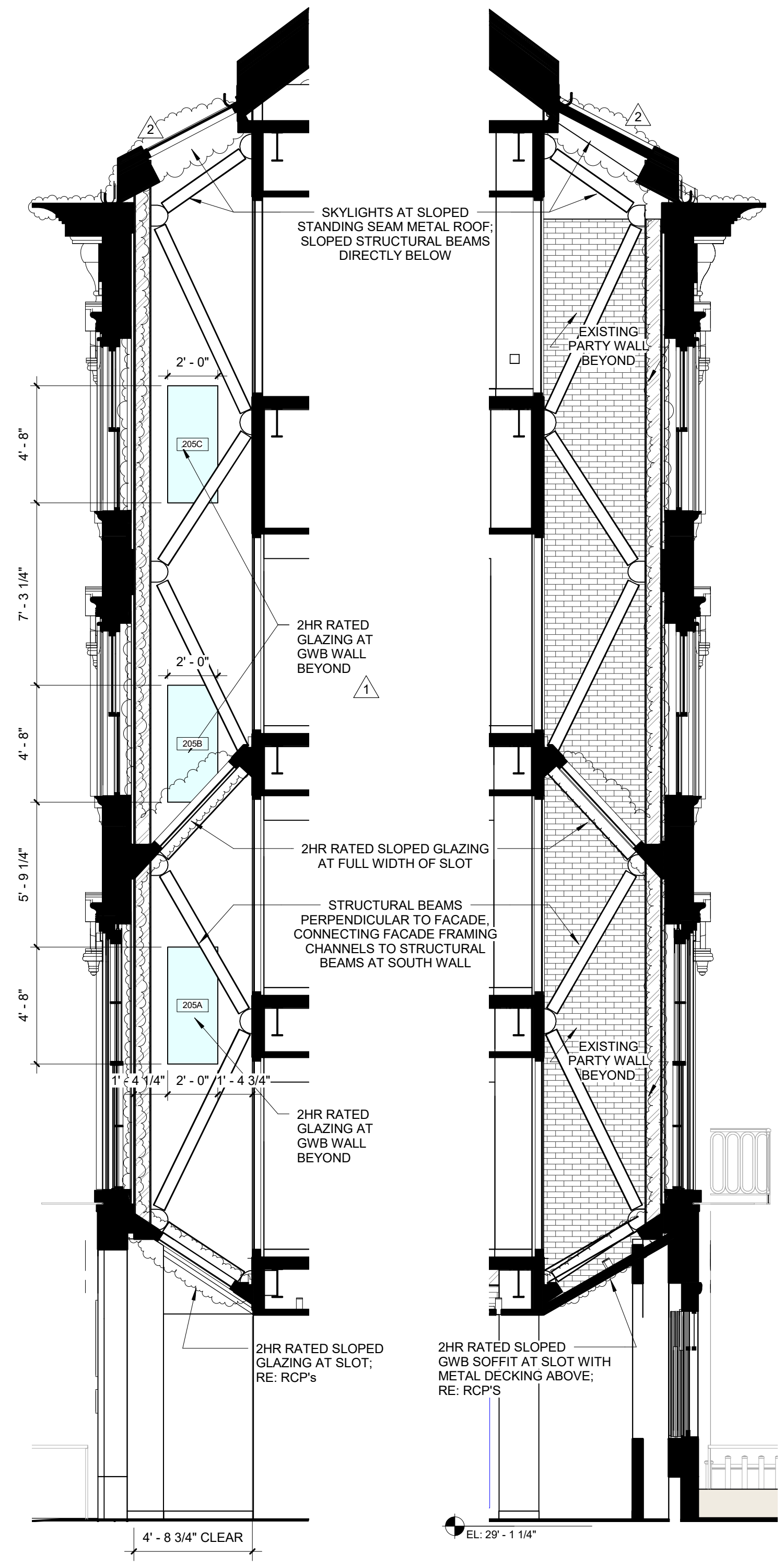
1 INTERIOR FACADE SLOT - EAST ELEVATION 1/4" = 1'-0"
