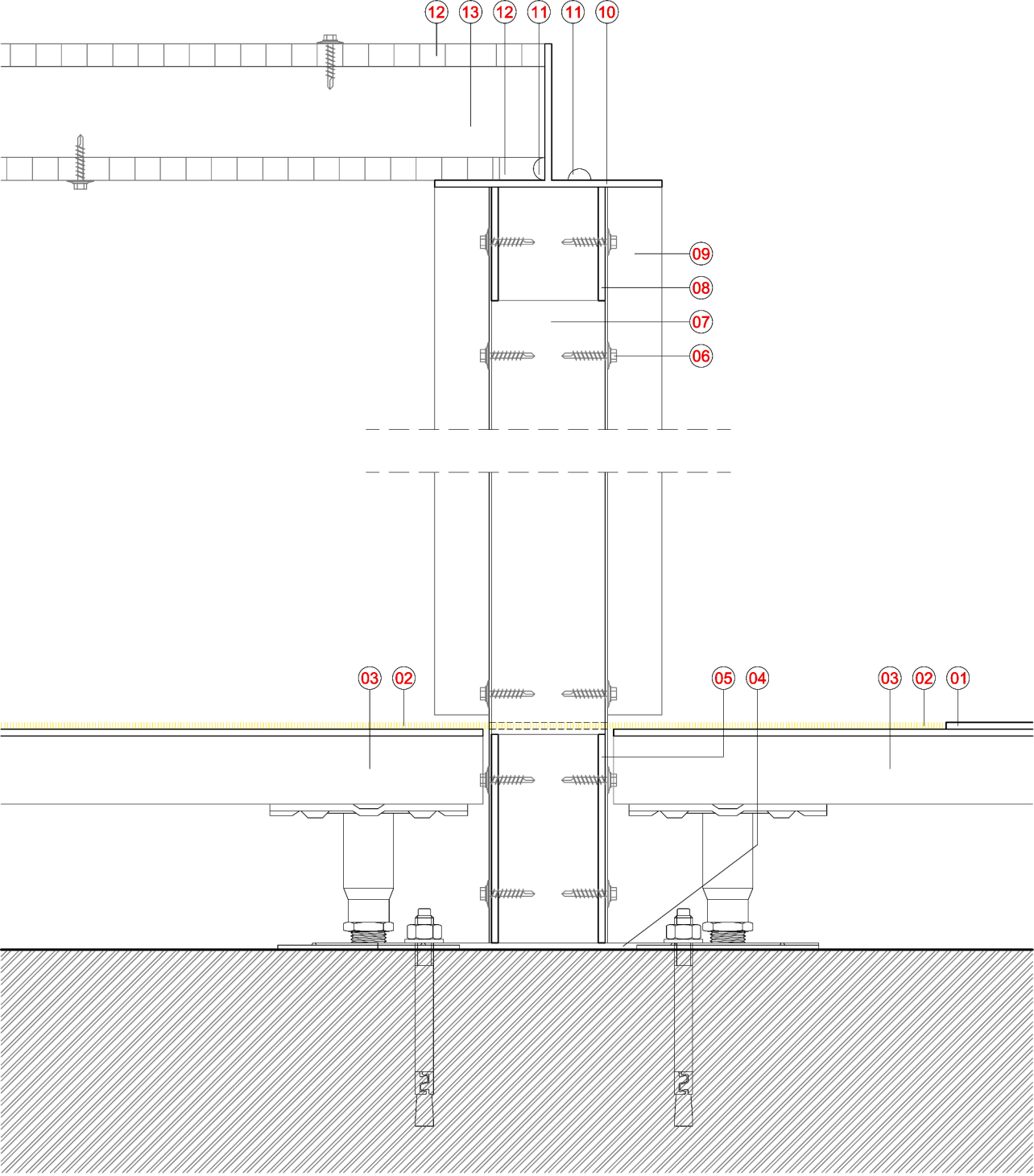
01.- VINYL FLOOR IN DARK GREY 02.- YELLOW CARPET 03.- EXISTING ACCESS FLOORING 04.- STEEL PLATE SCREWED TO SLAB 05.- STEEL TUBE Ø45.3 WELDED TO STEEL PLATE 06.- METHACRYLATE SCREW 07.- METHACRYLATE TUBE Ø50mm 08.- STEEL TUBE Ø45 WELDED TO TOP STRUCTURE 09.- ONDULATED POLYCARBONATE PANEL (SHINY SIDE OUTWARDS, ROUGH SIDE INWARDS) 10.- 3mm 'T' SHAPE STEEL STRUTURE PAINTED WHITE 11.- LED LIGHTING 12.- CELLULAR POLYCARBONATE PANEL SCREWED TO STRUTURE 13.- STEEL TUBE 40x40.3
