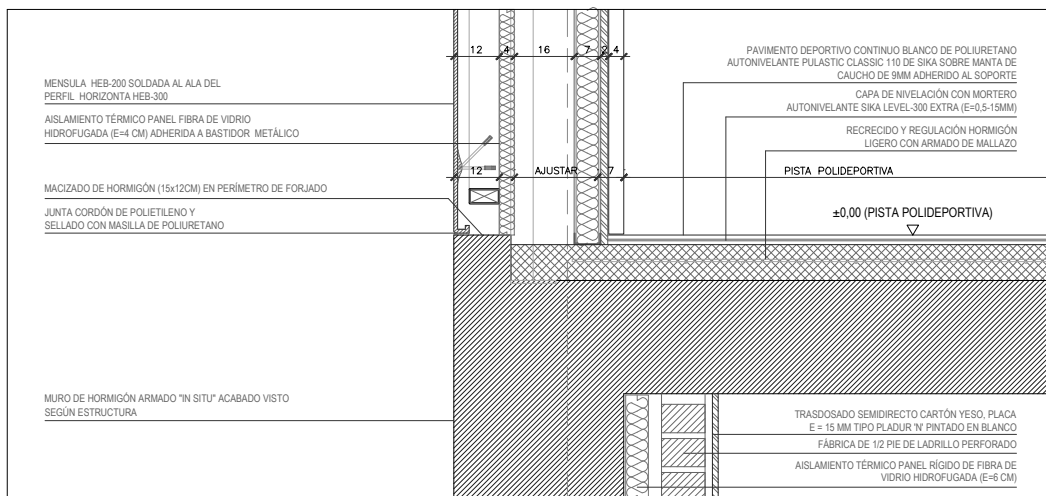
DETALLE ARRANQUE PANEL GRC
